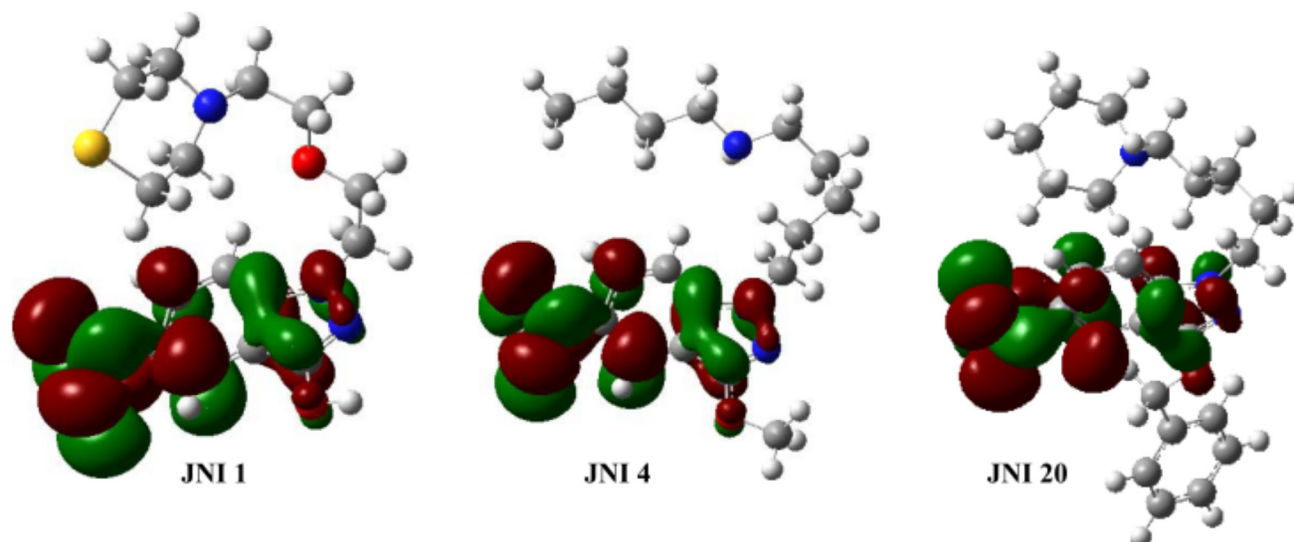
Figure 4. LUMO orbital distribution on compounds: JNI 1 (inactive), JNI 4 (medium activity) and JNI 20 (active).
