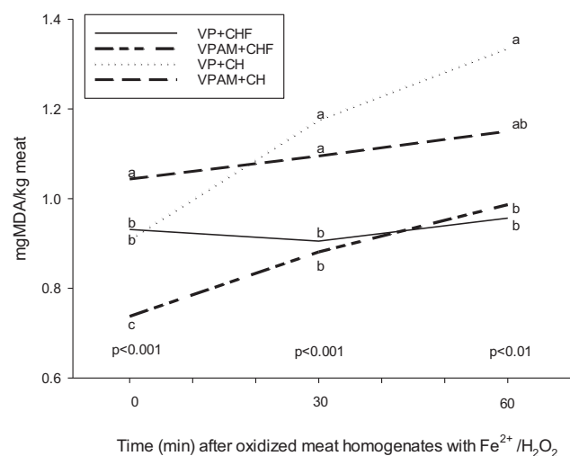
Figure 1. Resistance to oxidation during 60 min, expressed as TBARS level (mg MDA kg -1 meat) in beef homogenates oxidized by Fe 2+ /H 2 O 2 treated with different packaging and processes at 120 days of aging. VP + CH, vacuum packaging and chilled for 120 d; VP + CHF, vacuum packaging and chilled for 28 d and then frozen for 92 d; VPAM + CH, vacuum packaging with antimicrobial and chilled for 120 d; VPAM + CHF, vacuum packaging with antimicrobial and chilled for 28 d and then frozen for 92 d. Means with different letters at the each time point differ significantly ( P < 0.05 ).
